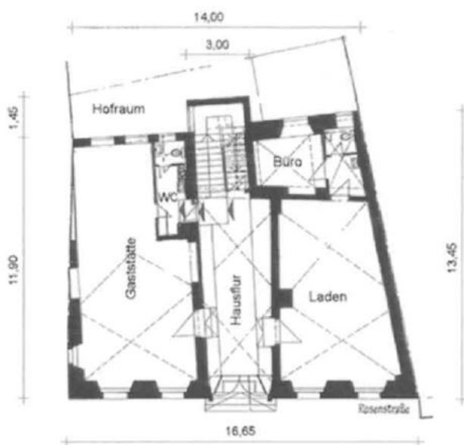
Grundriß Erdgeschoß
