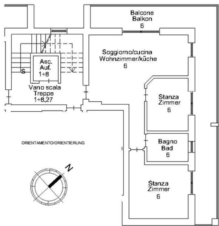
PIANO SECONDO - 2. STOCK
