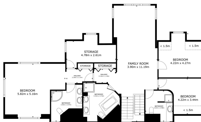
FLOOR 3
